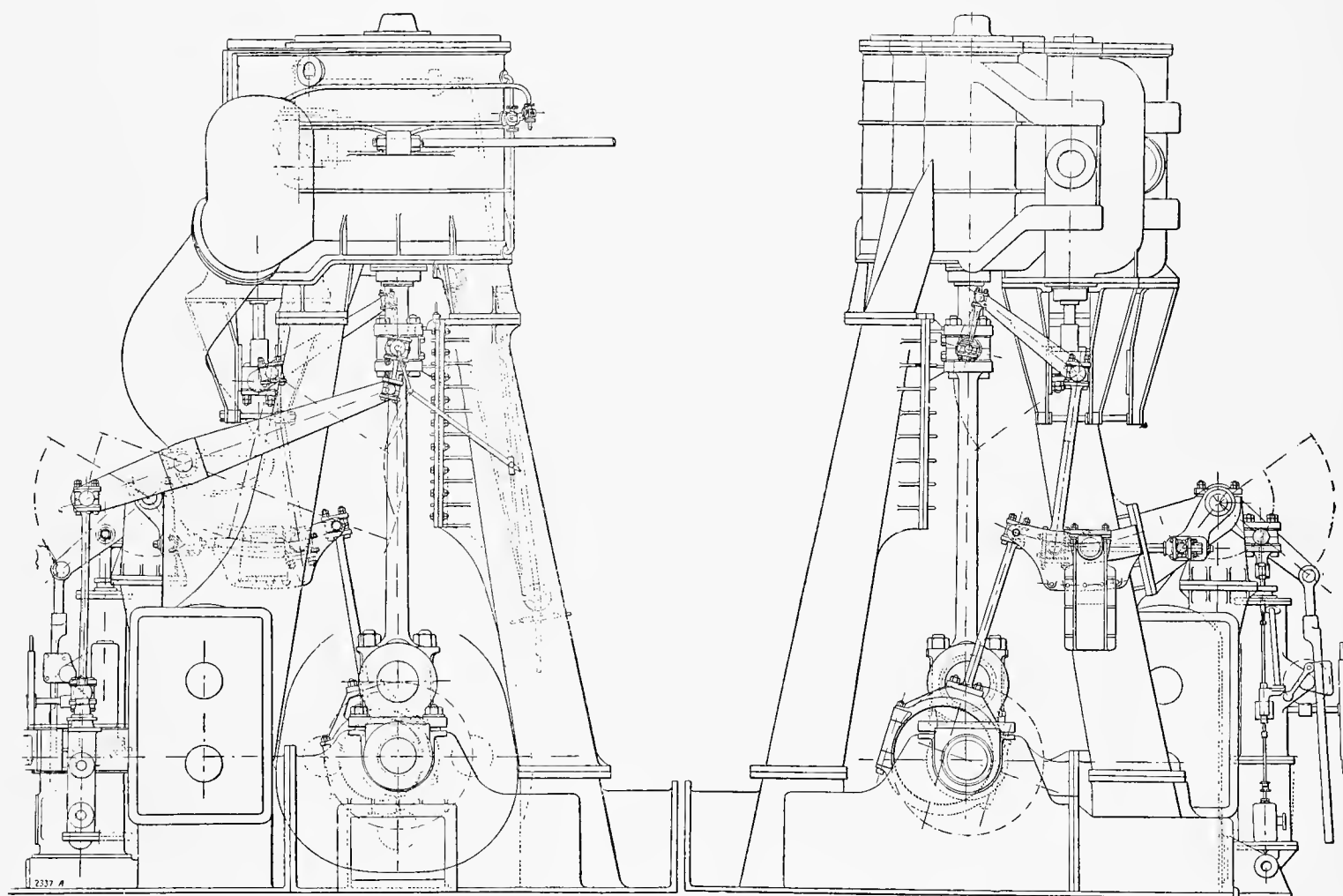
DRAWINGS OF END VIEWS OF ENGINES OF THE KENSINGTON.
